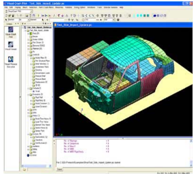
Software Screenshot
