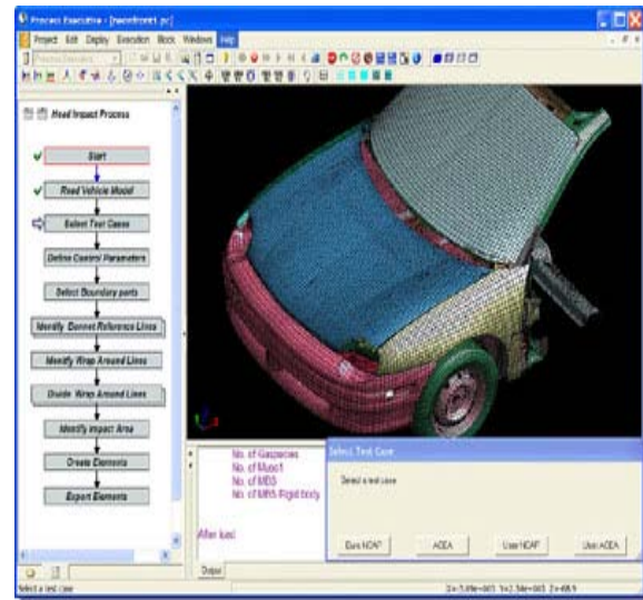
Software Screenshot
