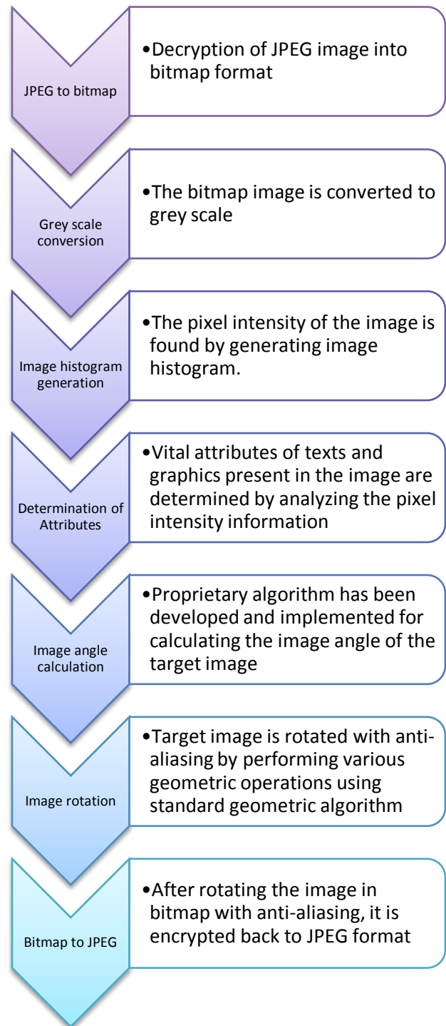
Image de-skew workflow
